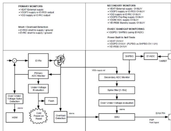
Power Supply Levels and Voltage Monitoring
