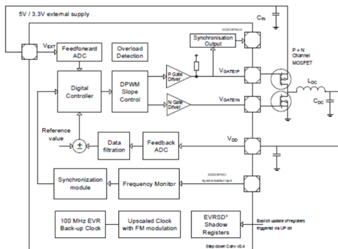
Step-Down Regulator
